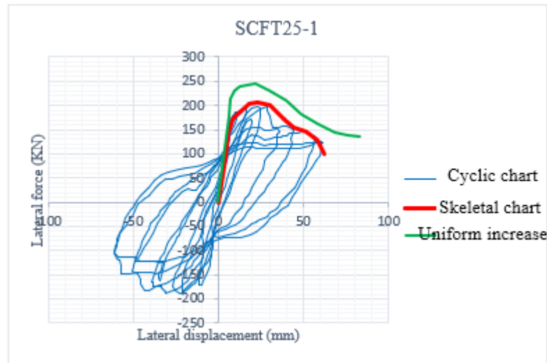
Figure 5. Force-displacement diagram of specimen SC.F.T25-1
